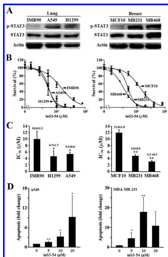
Figure 4. InS3-54 inhibits cancer cell proliferation. (A) Level of STAT3 expression and activation in different cells. Actin was used as a loading control. (B, C) Cytotoxicity assay. IC 50 of inS3-54 for each cell line was derived, and dose–response curves were created using PrismPad program. (D) Apoptosis assay of exponentially growing A549 and MDA-MB-231 cells. (** p < 0.01; * p < 0.05)
